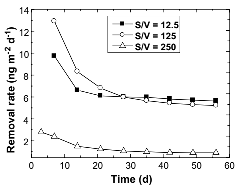
Fig. 3. Powder leaching results on perlite charged by 10 wt% in Cs 2 O.
