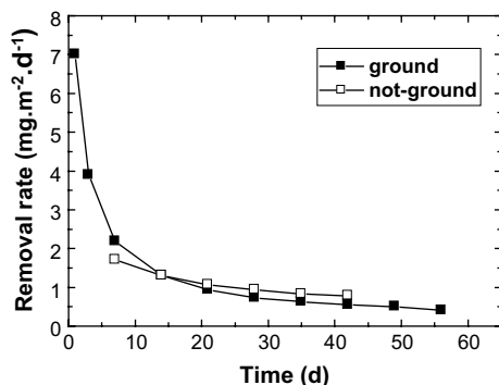
Fig. 6. Dynamic leaching test results on sintered samples.
