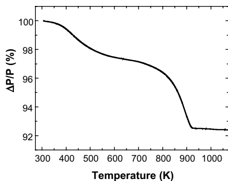
Fig. 1. TG-DTA traces of a 20 wt% sample.
